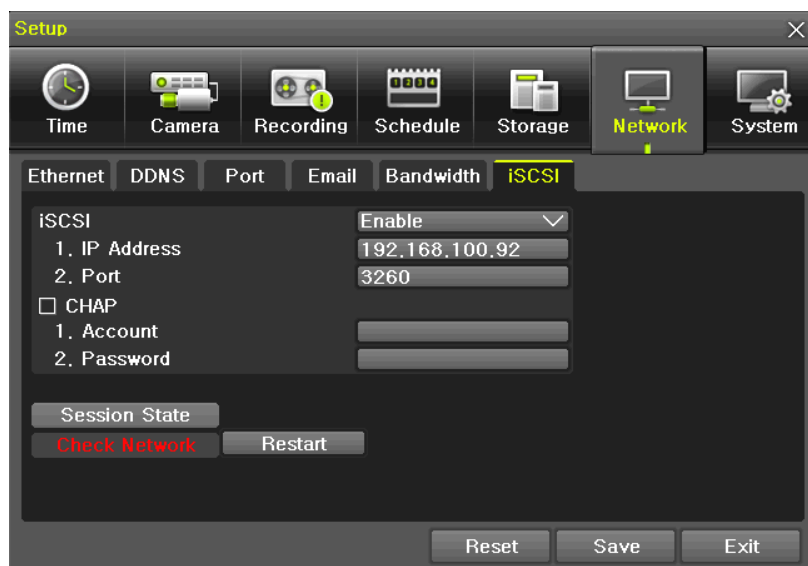
[Figure 6-50. Setup iSCSI Window1]
