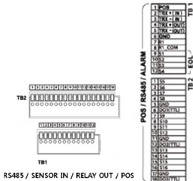
[Figure 2-2. COBRA ELITE 960H-16CH Terminal Block and Description]
