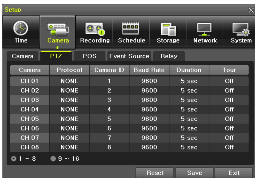
[Figure 5-11. PTZ Setup]
