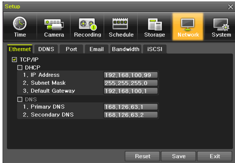
[Figure 6-47. Setup Network Ethernet Window]
