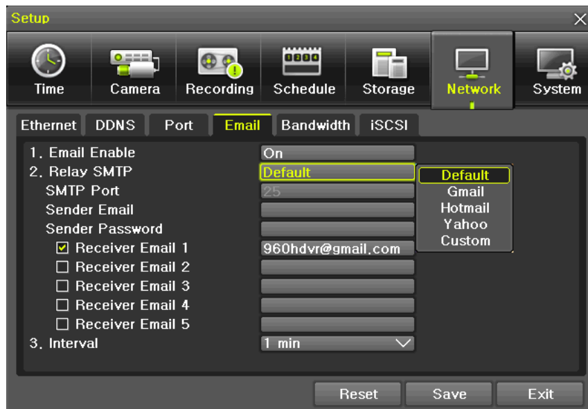
[Figure 6-48. Setup Network E-Mail Window1]
