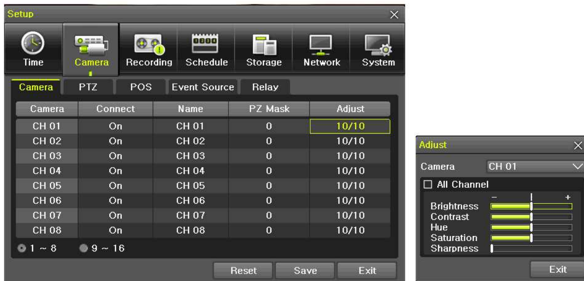
[Figure 5-15. Screen Setup Window]
