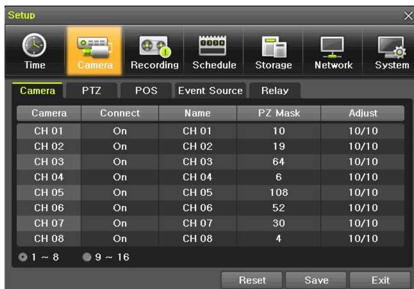
[Figure 6-40. Setup / Camera Menu]
