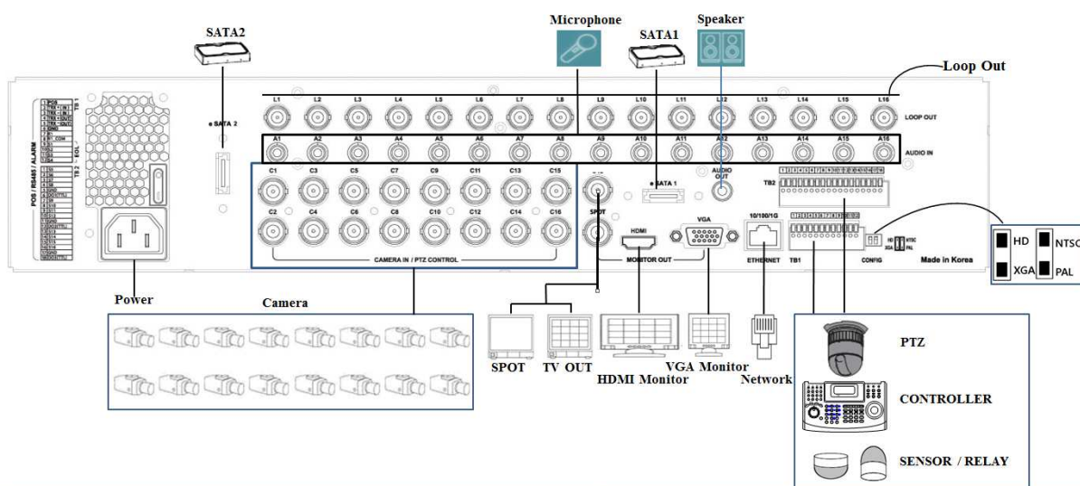
[Figure 2-1. COBRA ELITE 960H-16CH Basic Connection and Device Connection]
