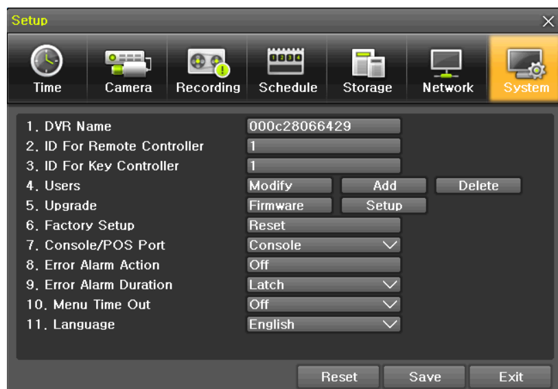
[Figure 6-52. System Setup Window]
