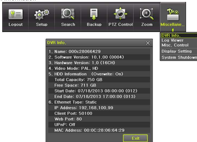
[Figure 5-14. Product Information Window]
