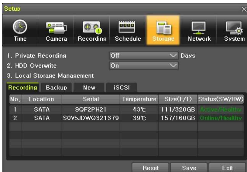
[Figure 6-44. Storage Window (Local)]
