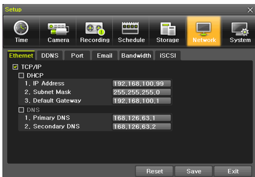
[Figure 6-45. Setup Network Window]
