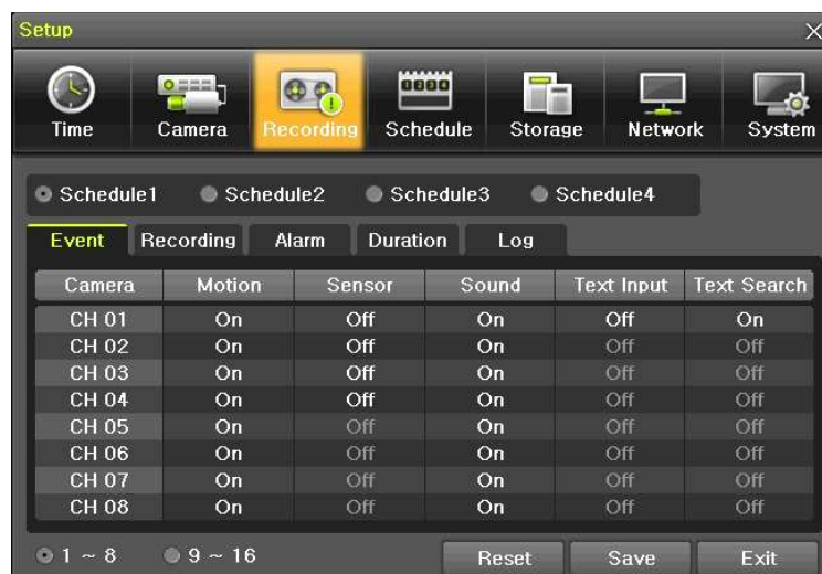
[Figure 6-42. Setup / Recording]
