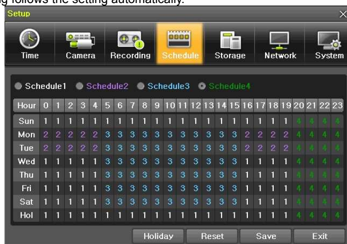
[Figure 6-43. Schedule Window]
